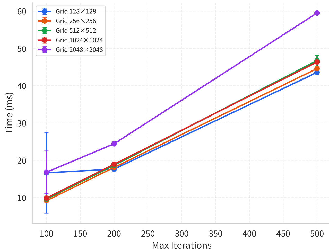
Jacobi 2D: Execution Time
