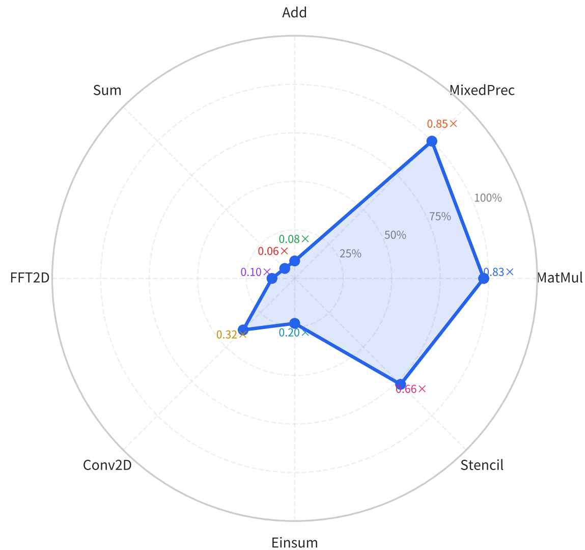
Normalized Speedup Radar (N=4096, 4 GPUs)
