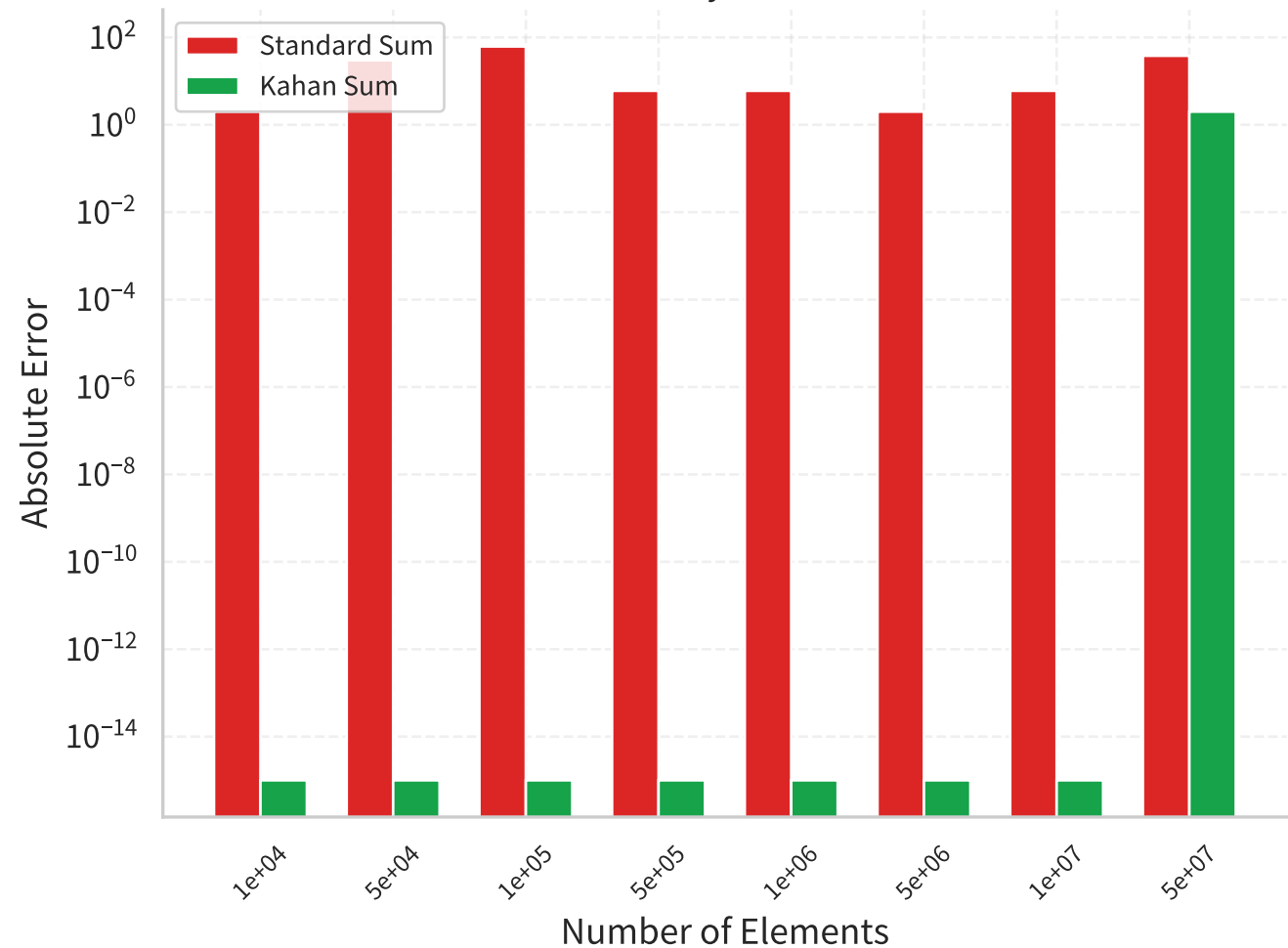
Numerical Accuracy: Standard vs Kahan
