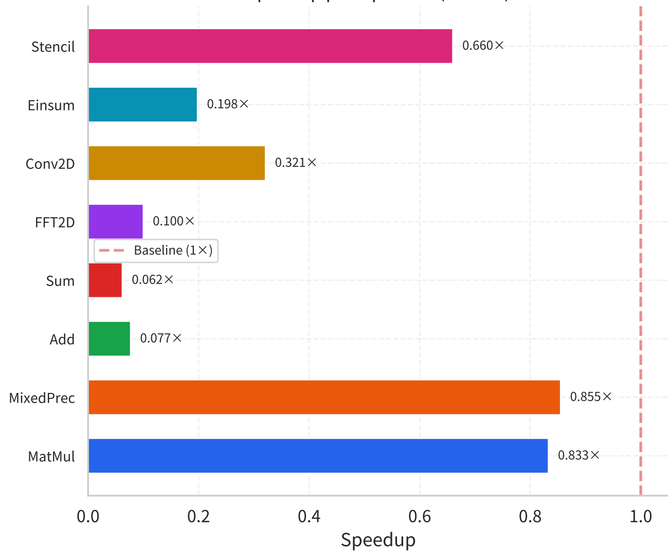
Speedup per Operator (4 GPUs)
