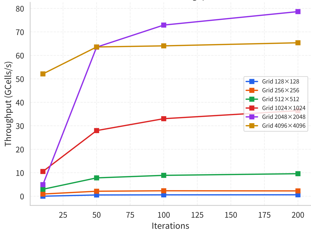
Stencil 2D: Throughput
