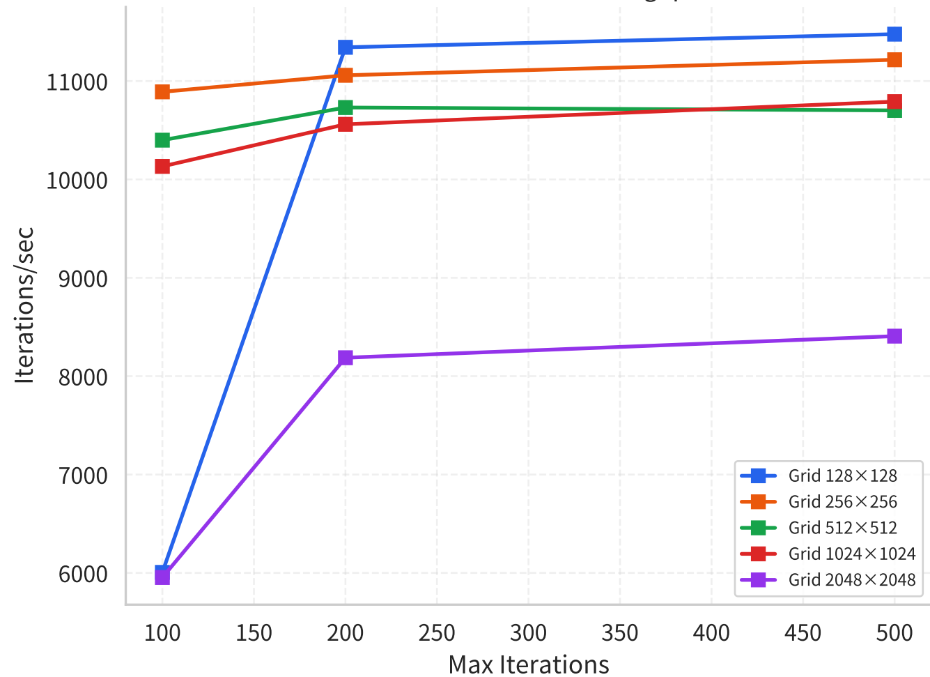
Jacobi 2D: Iteration Throughput
