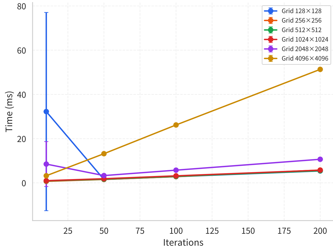
Stencil 2D: Execution Time
