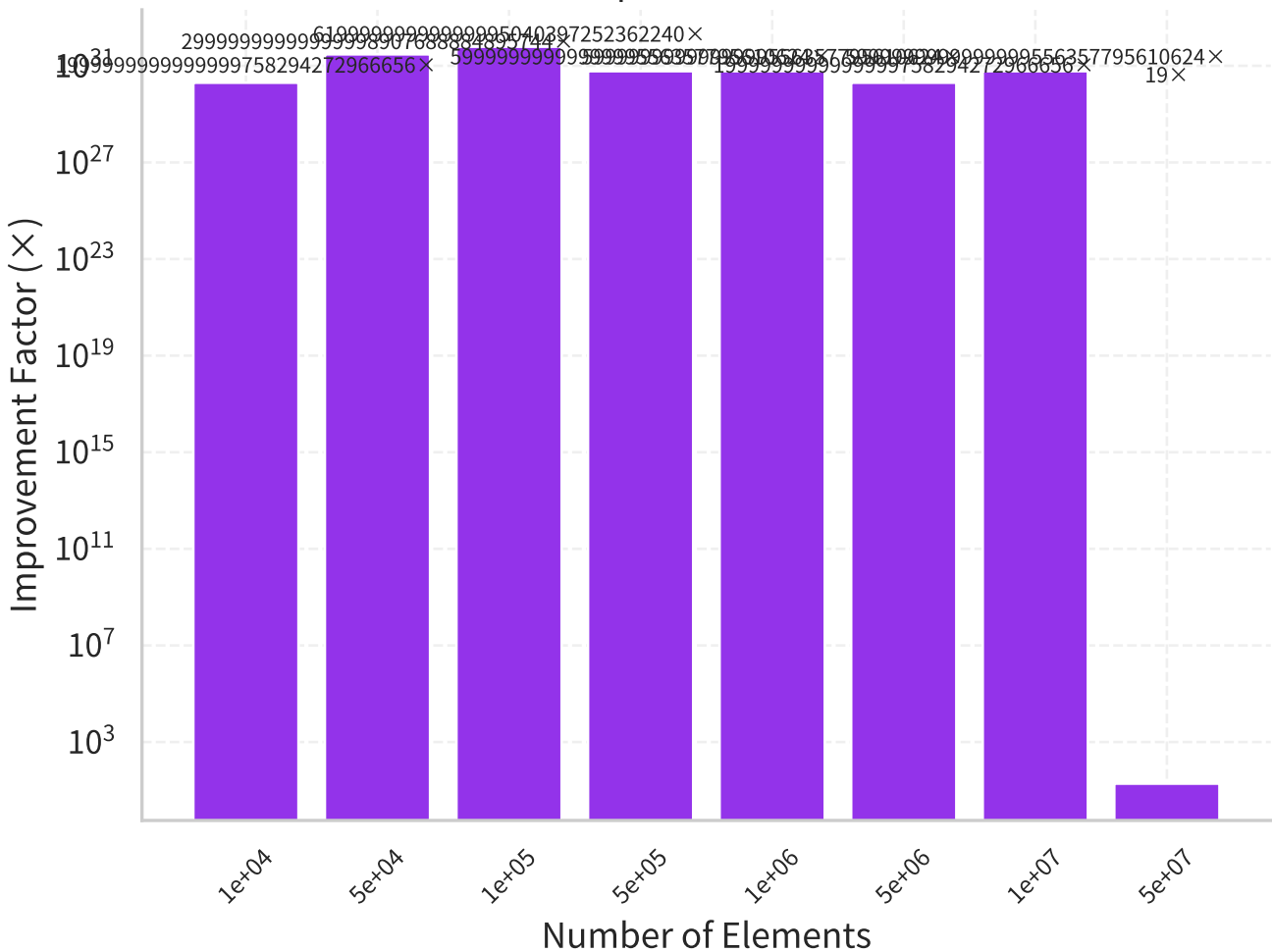
Kahan Sum Improvement over Standard
