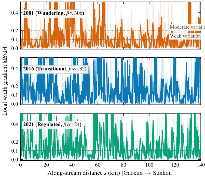
(a) Along-stream local width gradient |dB/ds| profiles
