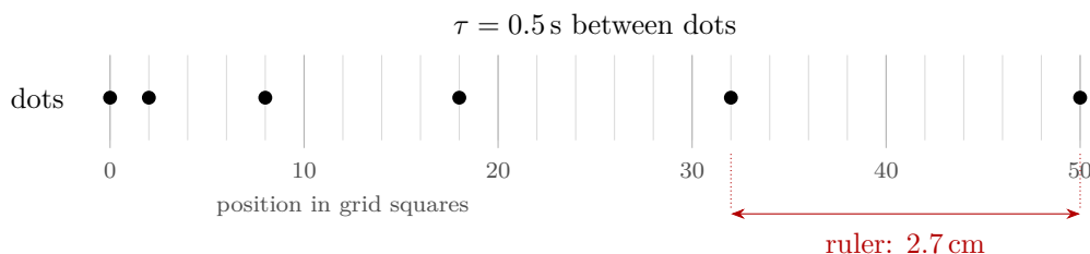
Figure 1.5: A dot diagram on a grid. Reading the dots gives the positions 0, 2, 8, 18, 32, 50 — in grid squares . One measurement converts the whole diagram: a ruler laid across the last gap, which spans 50 - 32 = 18 squares, reads 2.7 cm, so one square is 1.5 mm. Without that measurement the grid numbers have no physical size at all.
