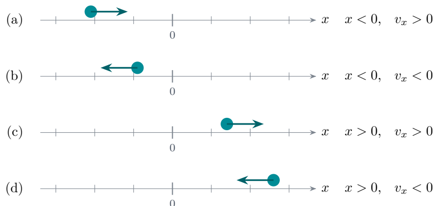
Figure 1.10: A skater at four moments. The dot gives the coordinate, the arrow gives the direction of travel. The sign of x and the sign of v_x are set independently, and all four combinations happen. In (a) the skater is to the left of the origin and moving right: the coordinate is negative and increasing , so the velocity is positive.
