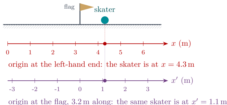
Figure 1.9: One skater, two coordinate systems. Measuring from the left-hand end of the track gives the coordinate x = 4.3 m; measuring from the flag gives x' = 1.1 m. The skater has not moved. What changed is the origin, and with it the bookkeeping: x' = x - 3.2 m at every point of the track.
