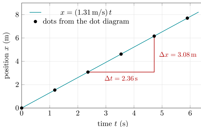
Figure 1.6: Position–time graph for a walker with 1.54 m strides every 1.18 s. The points fall on a straight line whose slope is the speed. The red triangle shows a rise of 3.08 m over a run of 2.36 s, a slope of 1.31 m/s.
