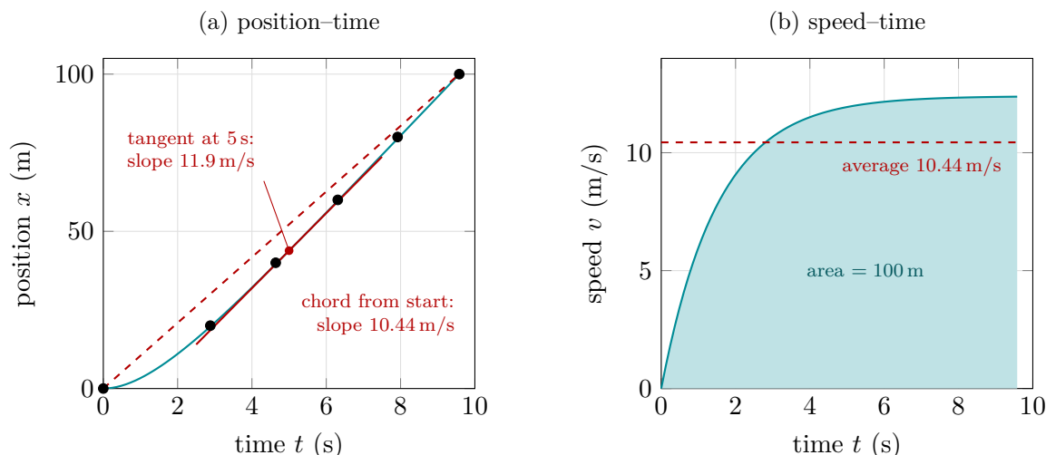
Figure 1.7: Bolt's world-record race. (a) Position against time: the dots are the measured 20 m split times and the curve is the model of Worked Example 1.10. The graph bends upward as he speeds up, then becomes nearly straight. The dashed chord from the start has slope equal to the average speed; the tangent at 5 s has slope equal to the instantaneous speed then. (b) The model's speed against time. The shaded area under the curve is the distance run, 100 m, and the dashed line is the average speed: a rectangle of that height has the same area as the curve.
