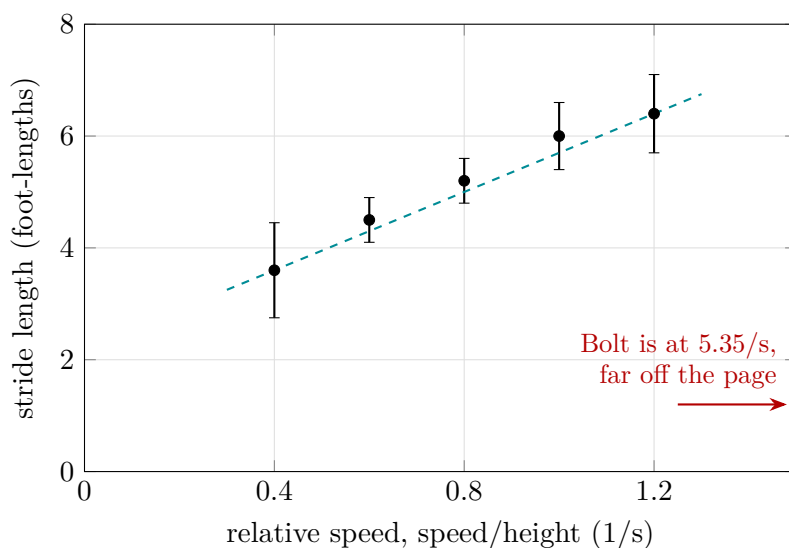
Figure 1.8: Schematic of the walking data behind the Charteris model, redrawn after Charteris, Wall, and Nottrodt (1981). Points show group means with a bar indicating the spread. The dashed line is a rough straight-line fit. The data stop at a relative speed of about 1.2/s.
