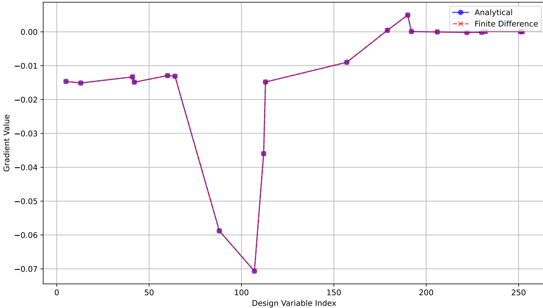
Max Stress Aggregation: Gradient Comparison
