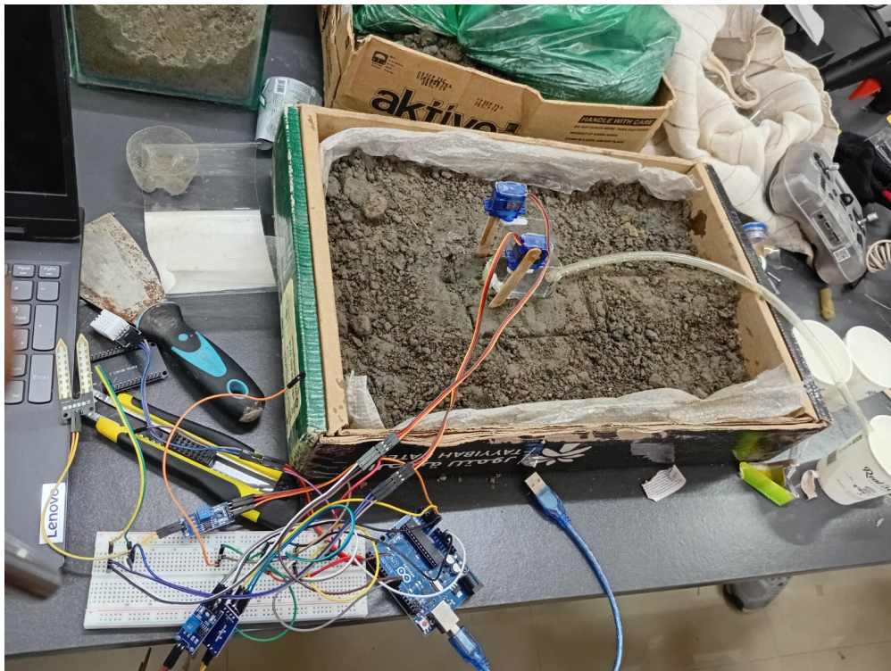
Figure 2: Ground Station setup for soil monitoring
