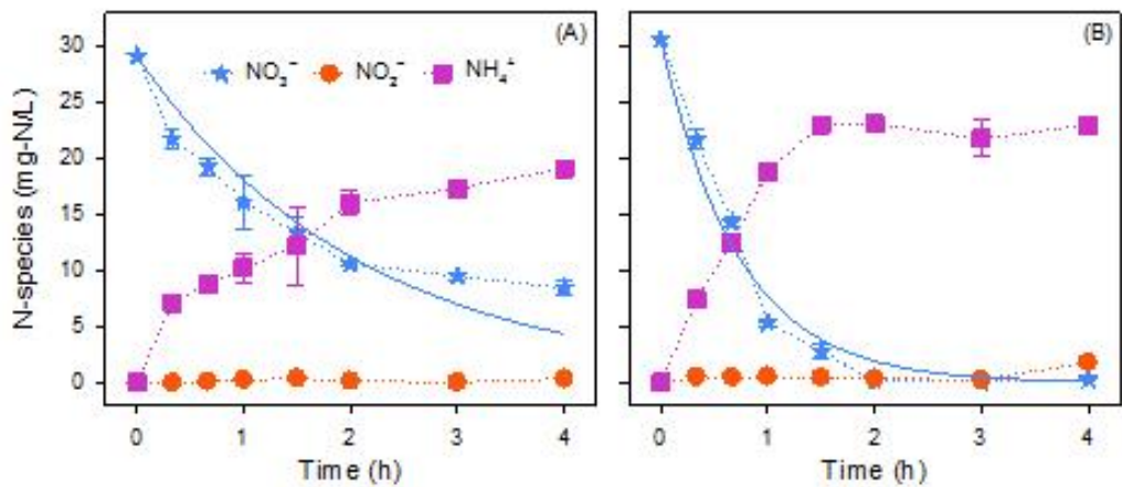
图 3-1 金属铜负载对纳米零价铁还原硝酸盐的影响 (A) nZVI, (B) 0.05%Cu-nZVI (反应条件: [\text{NaCl}]_0 = 1 \text{ mM} , [\text{KNO}_3]_0 = 2 \text{ mM} , \text{pH}_0 = 4.0 , [\text{nZVI}]_0 = 1 \text{ g/L} , T = 25 \text{ }^\circ\text{C} .)
