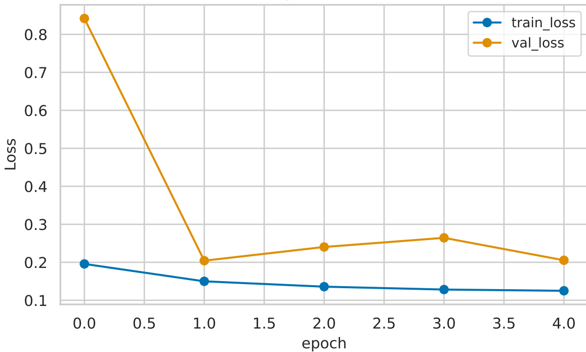
Training/Validation Loss
