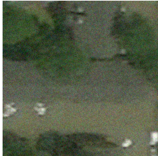
validation/damage,-95.648986_29.837208.jpeg
