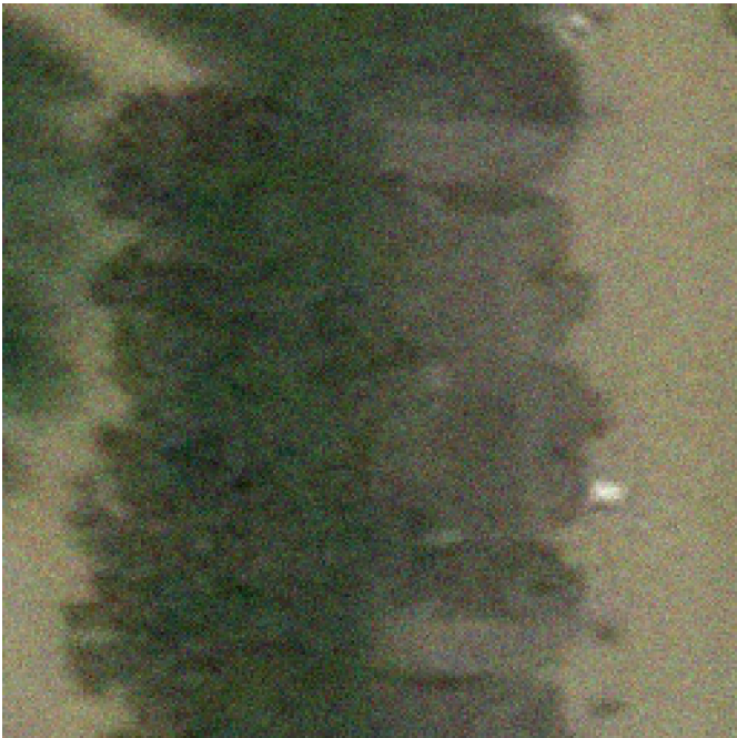
validation/damage,-95.623049_29.777490999999998.jpeg
