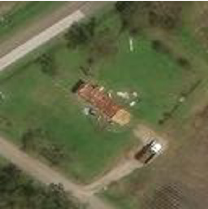
validation/damage,validation_damage_-96.90476600000001_28.3752116116.jpg,validation_damage_-96.907167_28.7639961616.jpg,validation_damage_-96.899902_28.761128999999997_f285cf.jpeg
