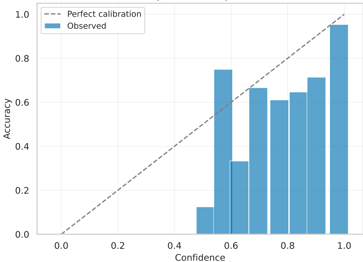
resnet34 | Test reliability (calibrated)
