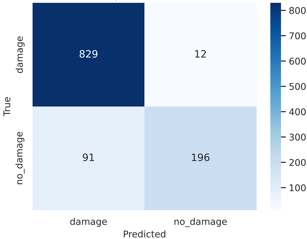
resnet34 | Test confusion (raw)
