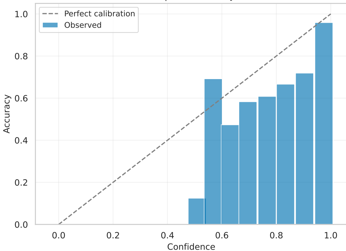
resnet34 | Test reliability (raw)
