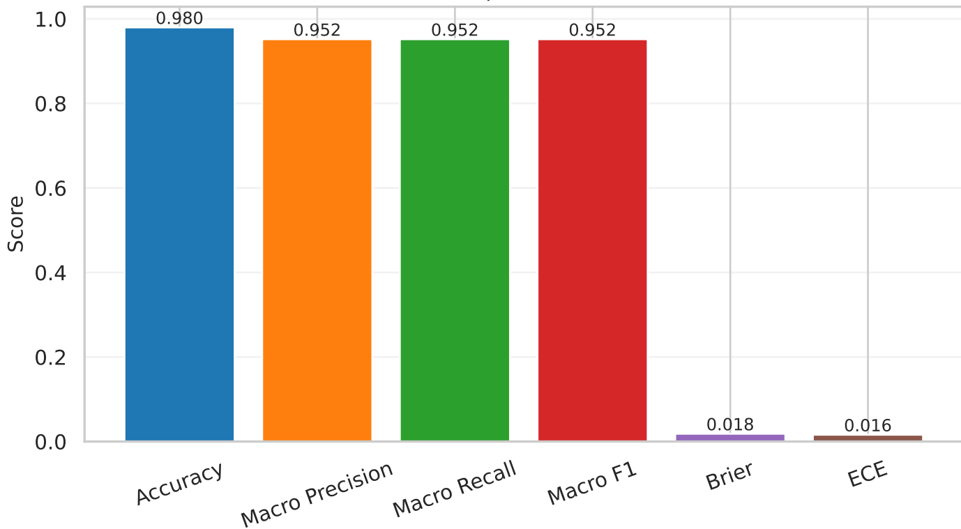
resnet34 | val (calibrated)
