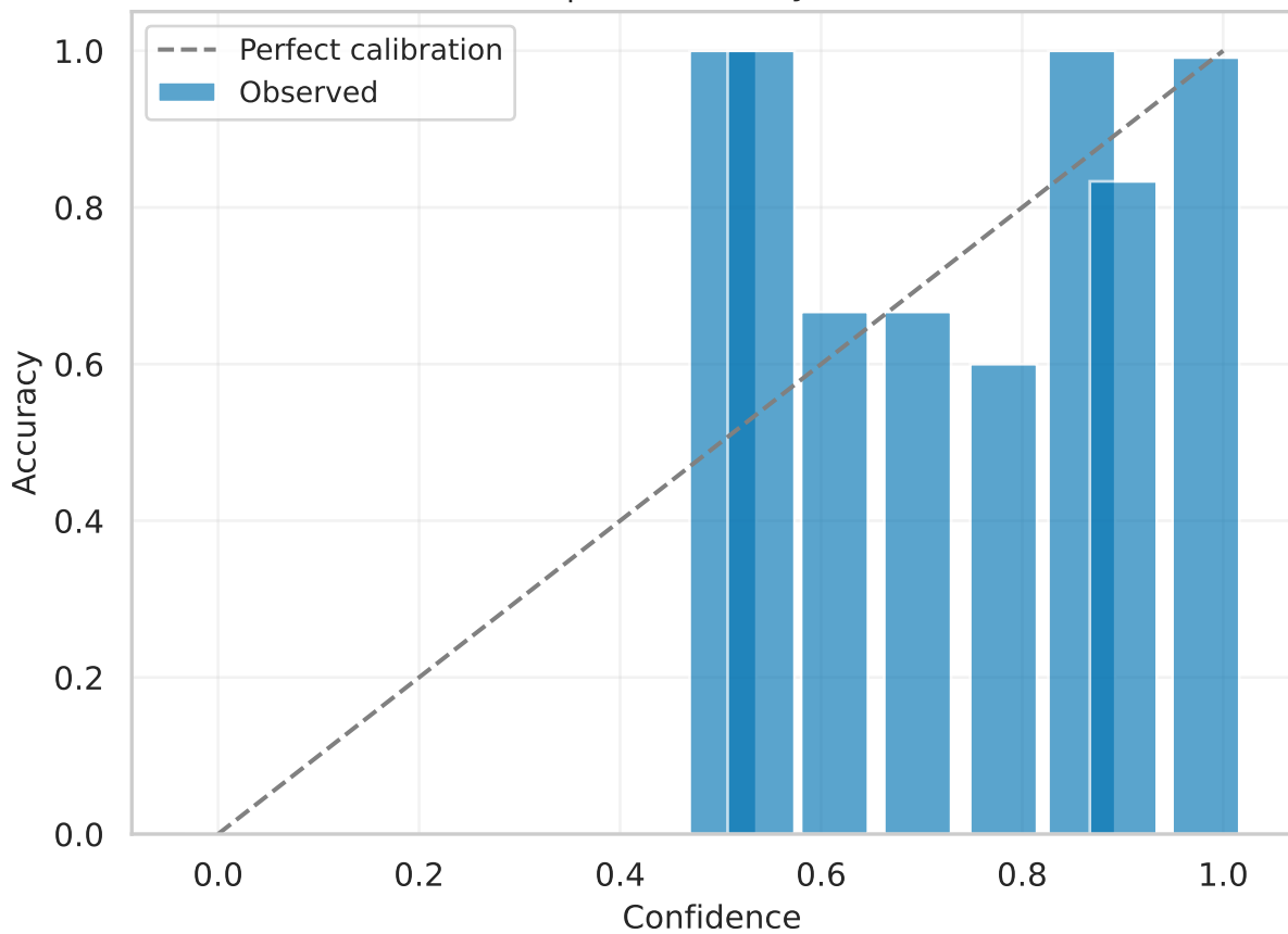
resnet34 | Val reliability (calibrated)
