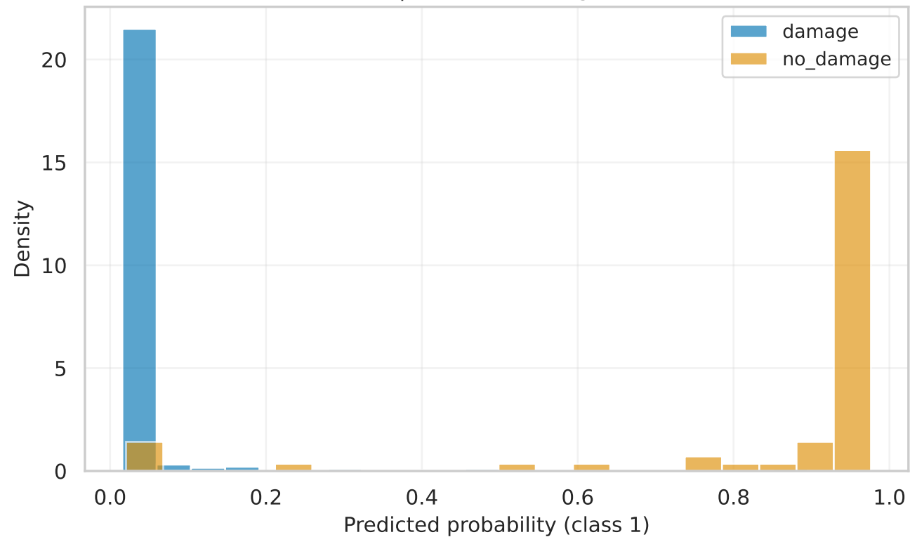
resnet34 | Val score histogram (raw)
