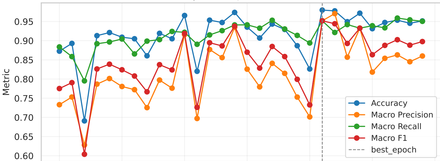
resnet34 | Accuracy/Precision/Recall/F1
