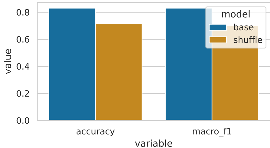
Key metrics
