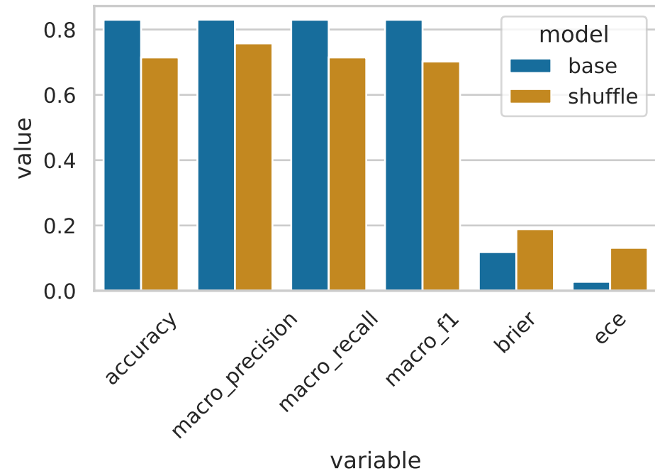
Test metrics
