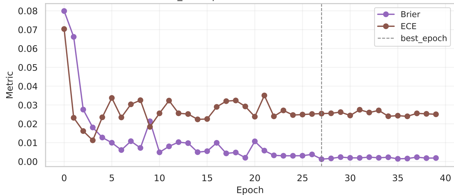
convnext_small | Calibration metrics (Brier/ECE)
