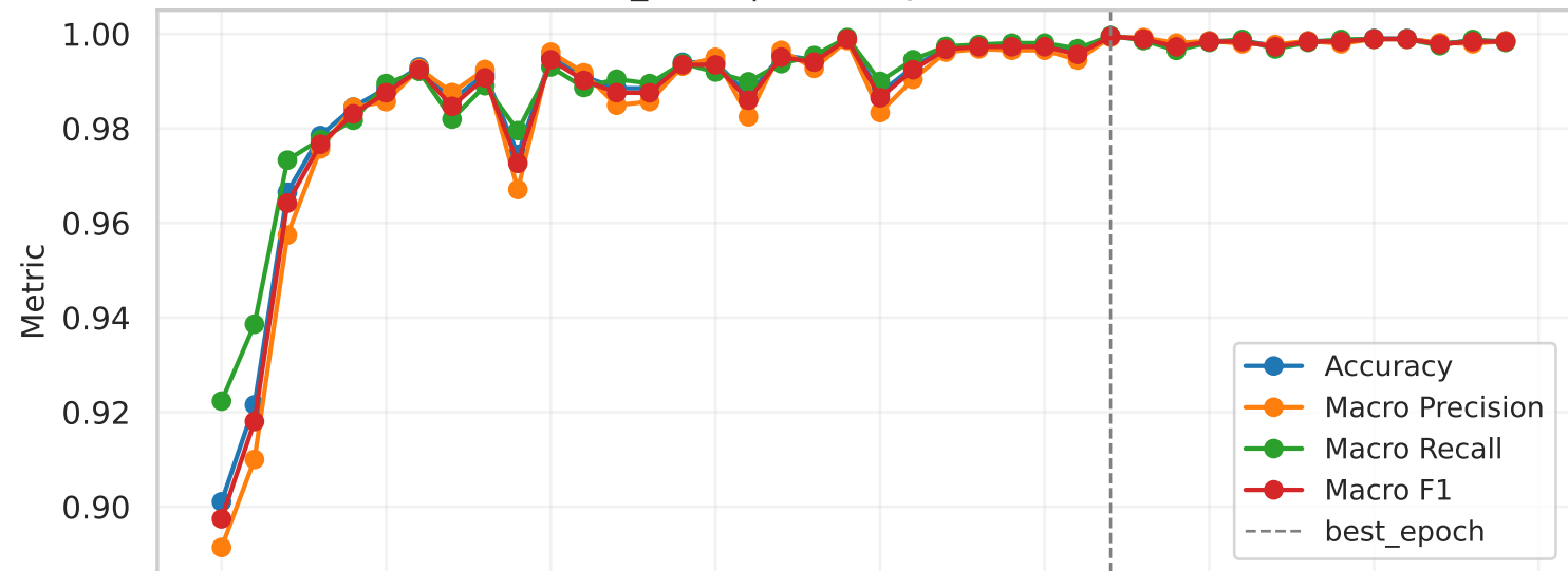
convnext_small | Accuracy/Precision/Recall/F1
