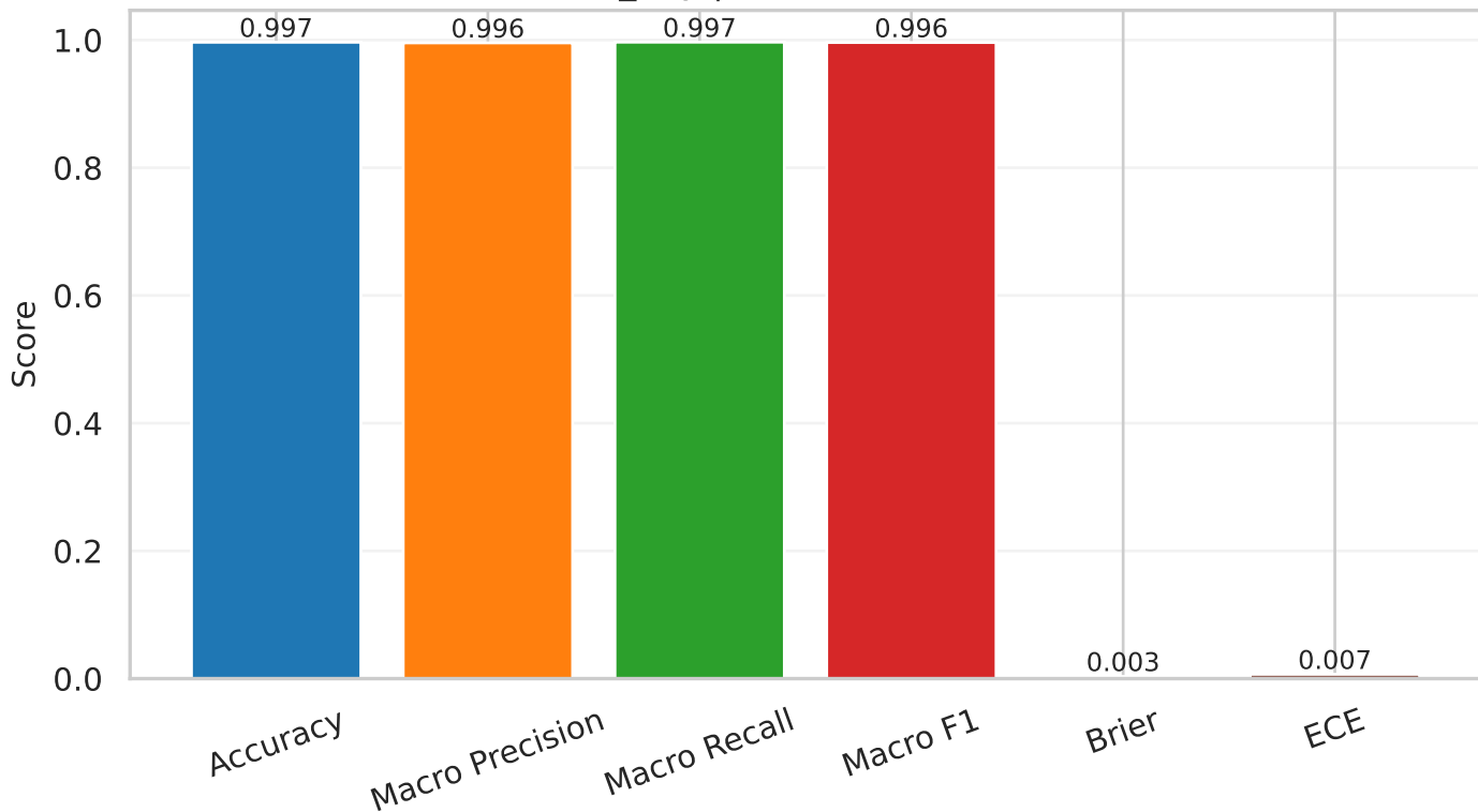
convnext_tiny | test (calibrated) metrics
