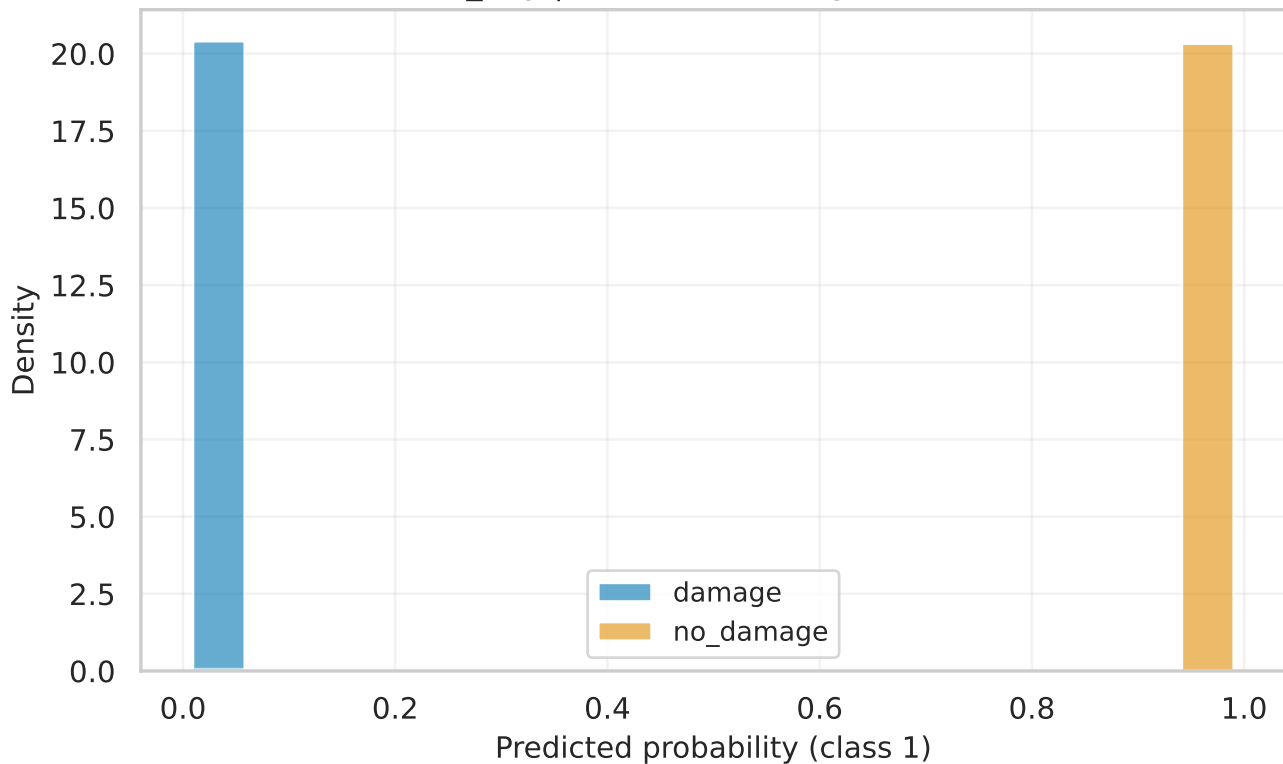
convnext_tiny | test Score Histogram (calibrated)
