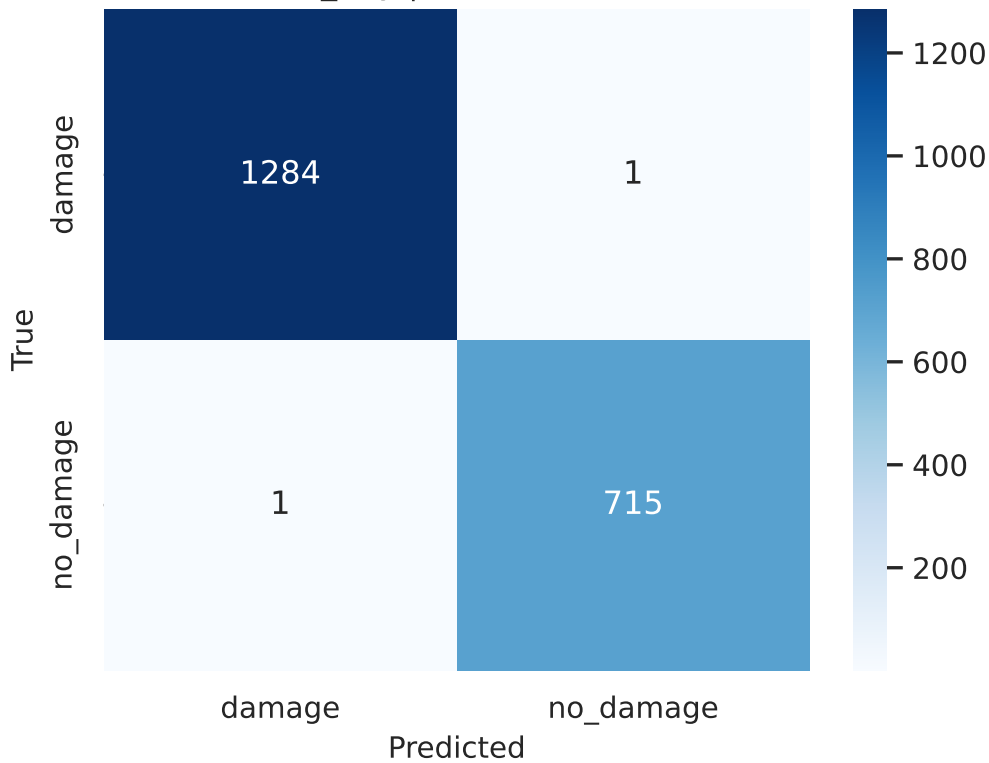
convnext_tiny | val Confusion (raw)
