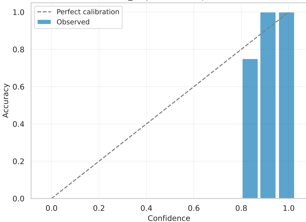
efficientnet_b1 | val Reliability (calibrated)
