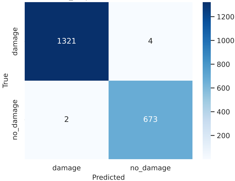
efficientnet_b2 | test Confusion (calibrated)
