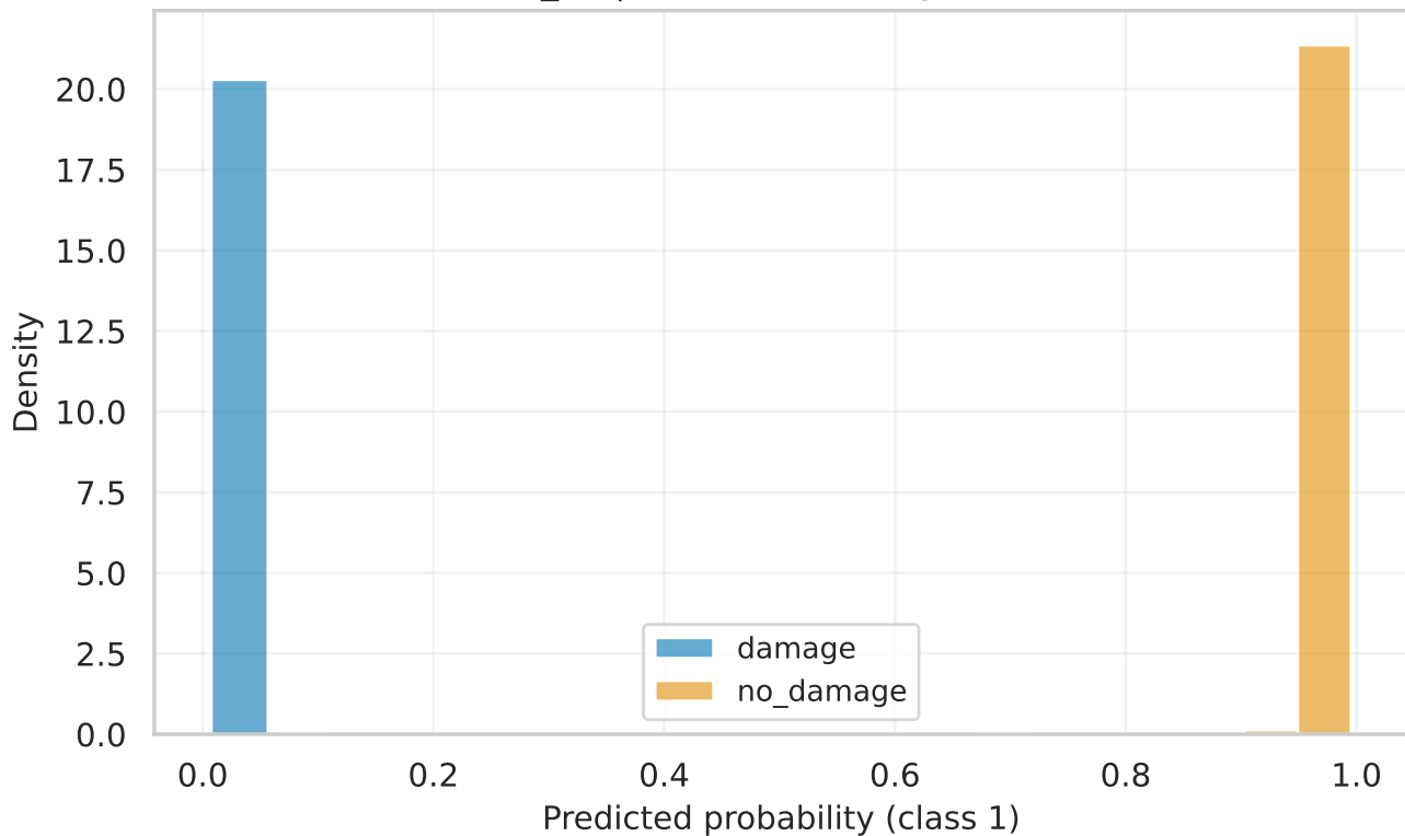
efficientnet_b2 | test Score Histogram (calibrated)
