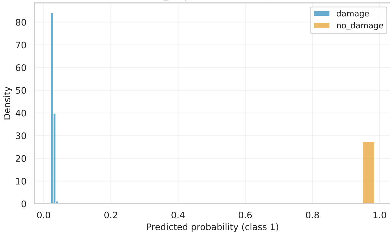
efficientnet_b2 | val Score Histogram (raw)
