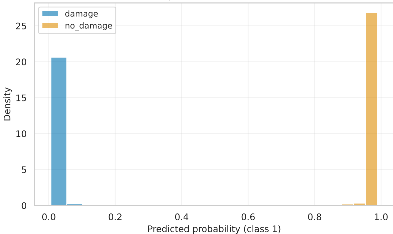
resnet18 | test Score Histogram (raw)
