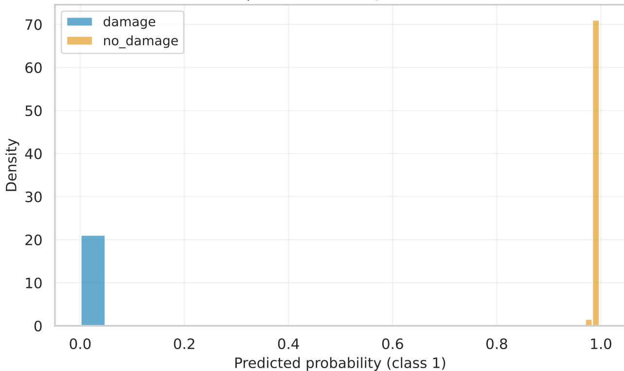
resnet18 | val Score Histogram (calibrated)
