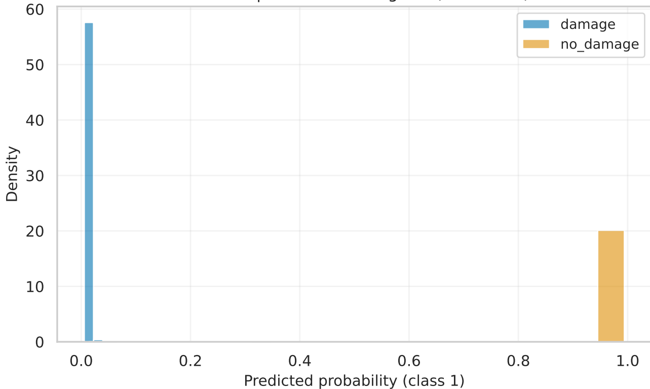
resnet34 | val Score Histogram (calibrated)
