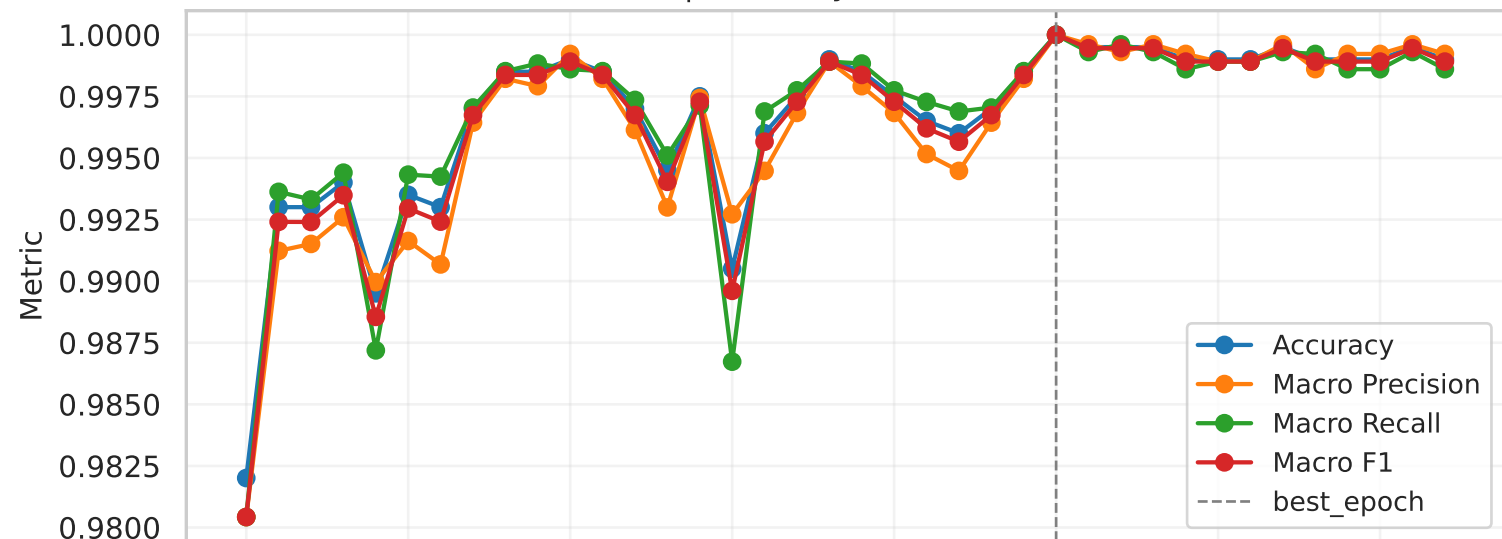
resnet50 | Accuracy/Precision/Recall/F1
