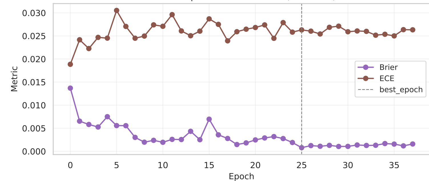
resnet50 | Calibration metrics (Brier/ECE)
