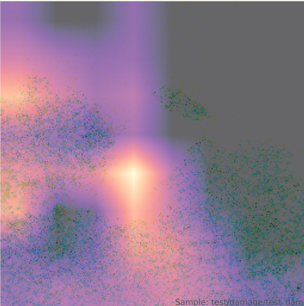
ConvNeXt-Tiny Damage confidence: 0.96
