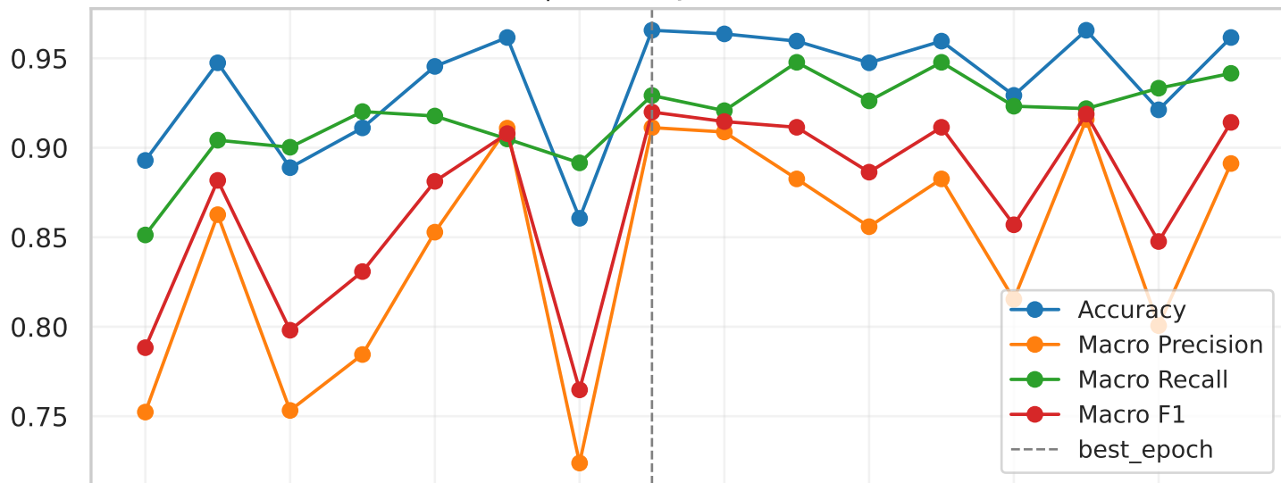
resnet34 | Accuracy/Precision/Recall/F1
