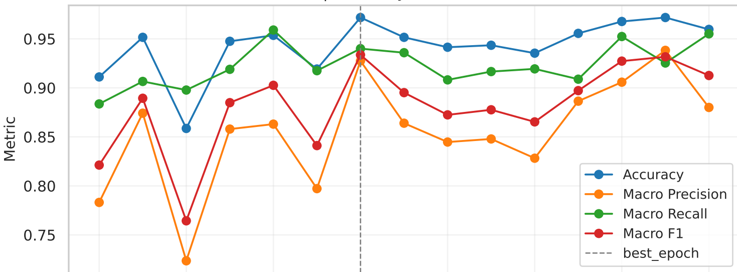
resnet34 | Accuracy/Precision/Recall/F1
