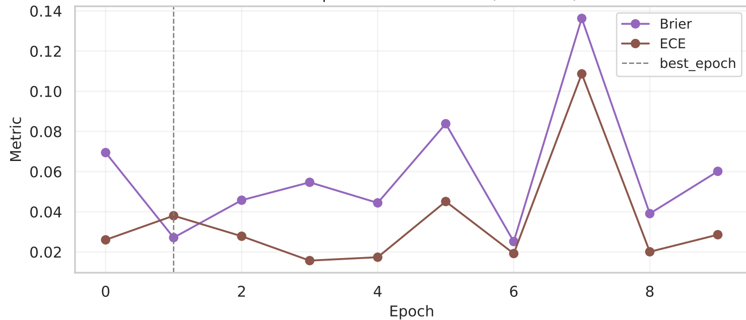
resnet34 | Calibration metrics (Brier/ECE)
