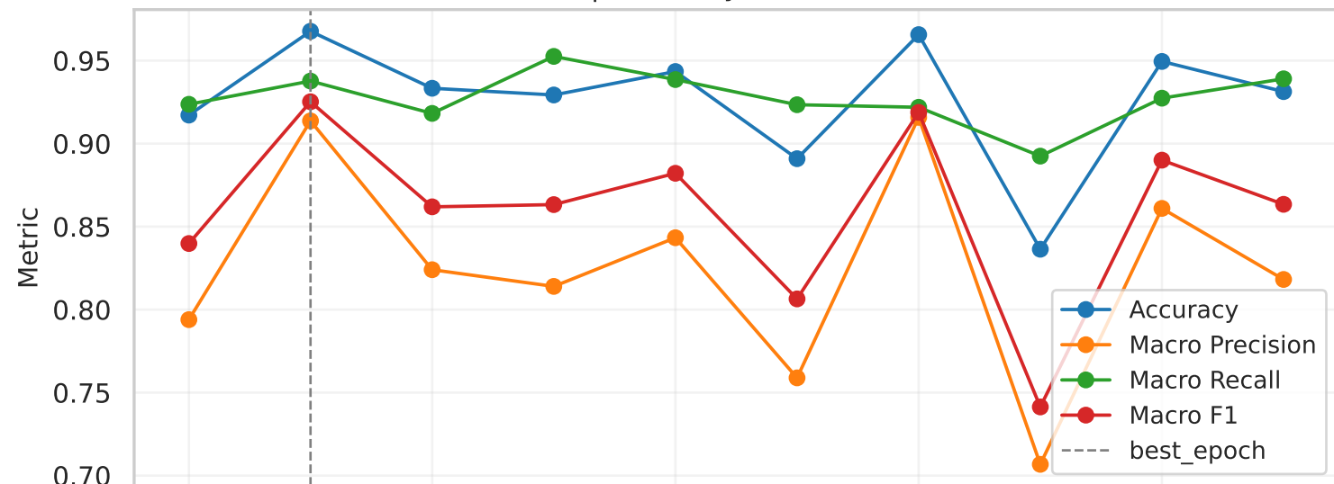
resnet34 | Accuracy/Precision/Recall/F1
