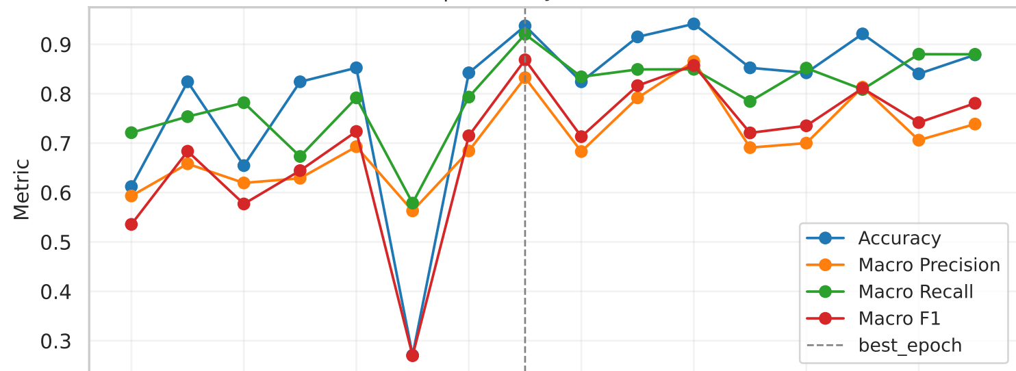
resnet34 | Accuracy/Precision/Recall/F1
