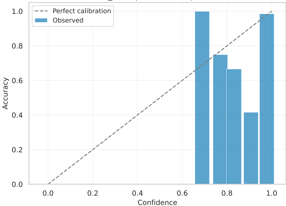
convnext_small | test Reliability (calibrated)
