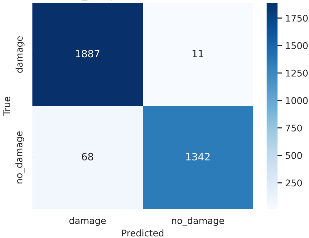
convnext_tiny | test Confusion (calibrated)
