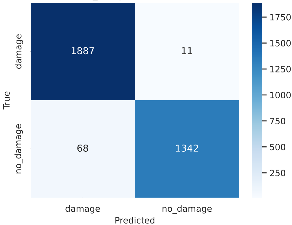
convnext_tiny | test Confusion (raw)
