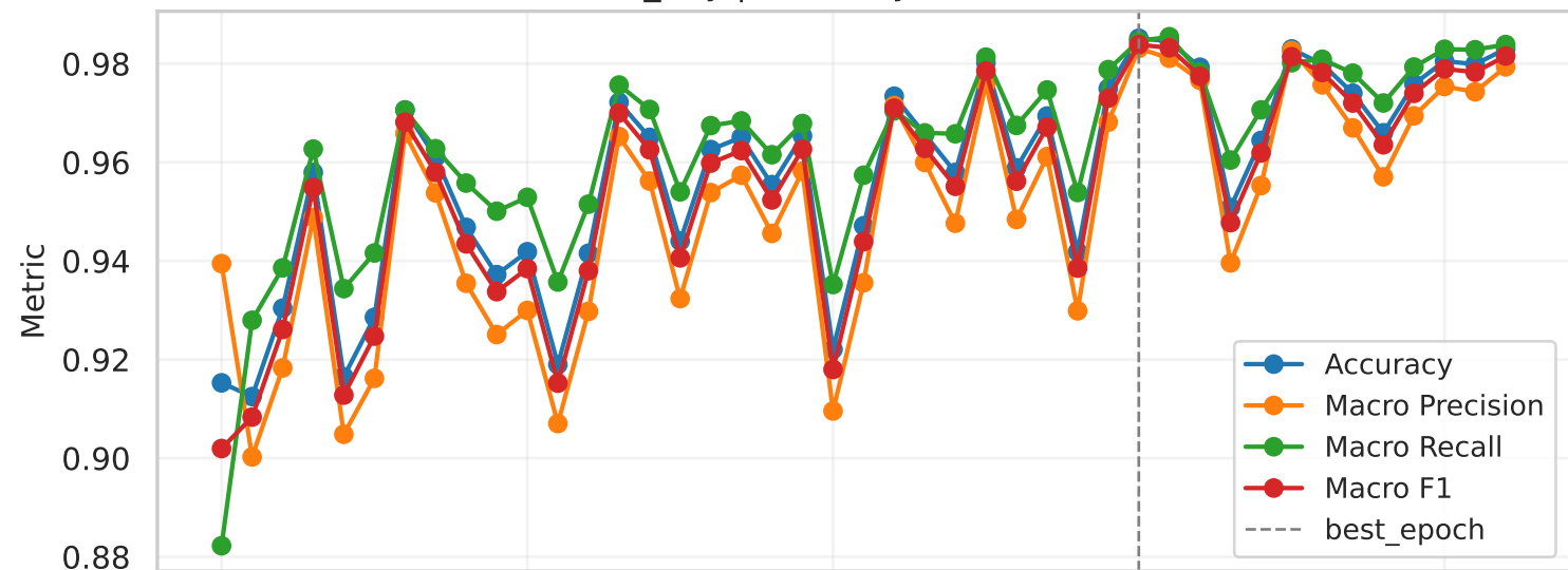
convnext_tiny | Accuracy/Precision/Recall/F1
