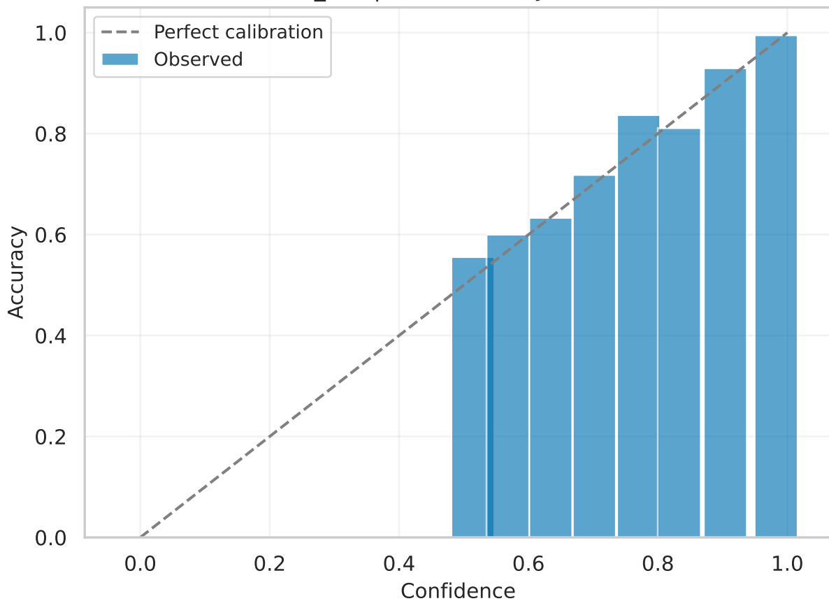
custom_cnn | test Reliability (calibrated)
