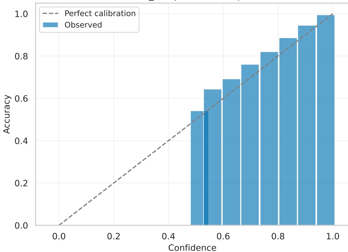
custom_cnn | val Reliability (raw)
