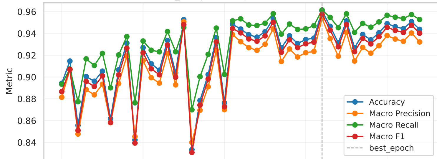
custom_cnn | Accuracy/Precision/Recall/F1
