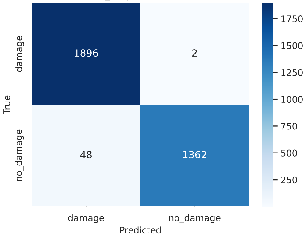
efficientnet_b1 | test Confusion (raw)
