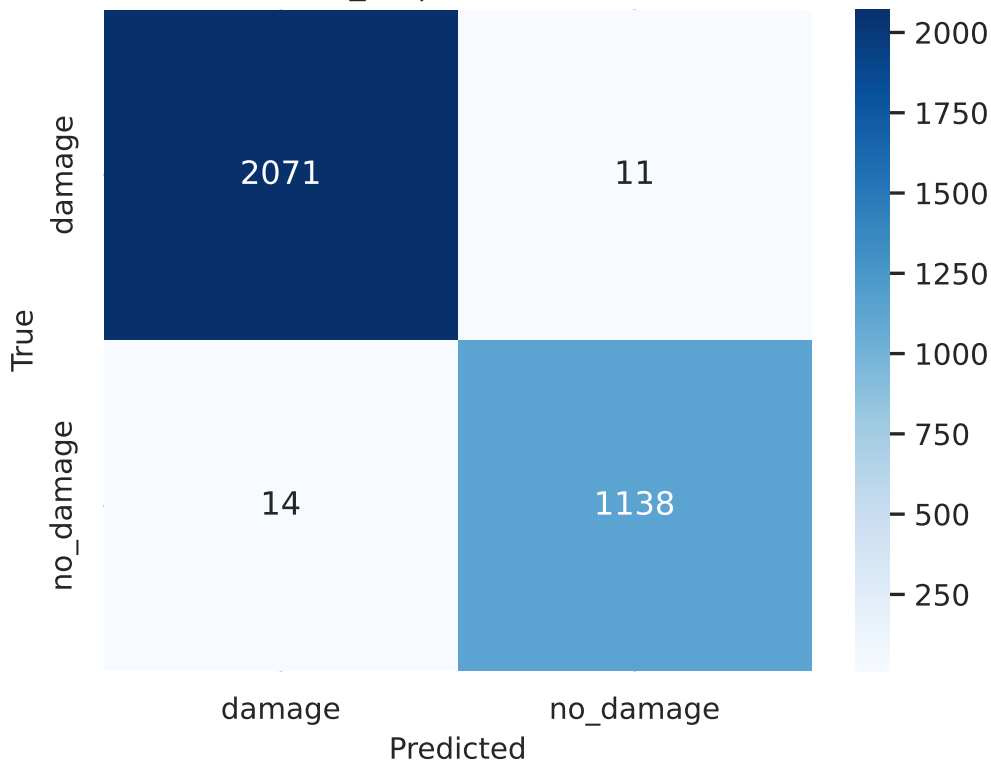
efficientnet_b1 | val Confusion (raw)
