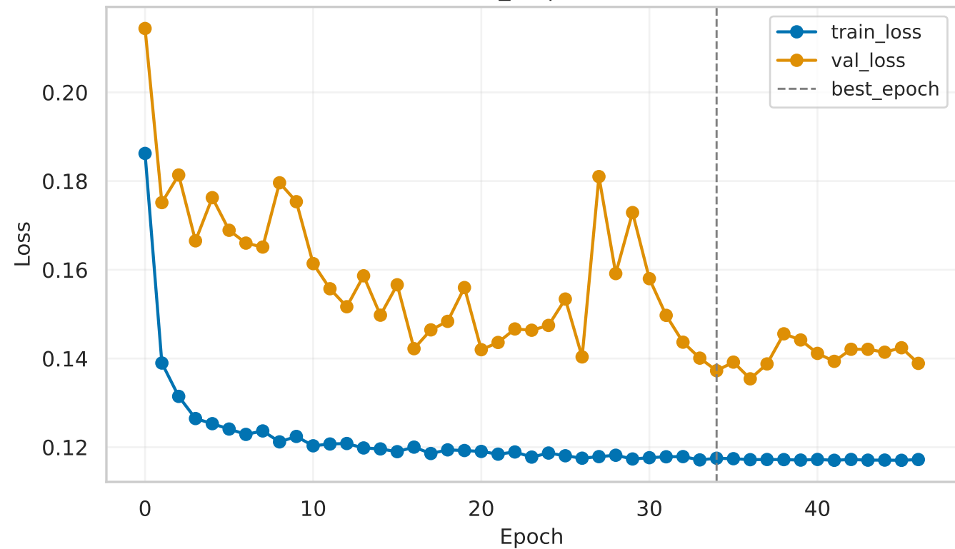
efficientnet_b1 | Loss curves
