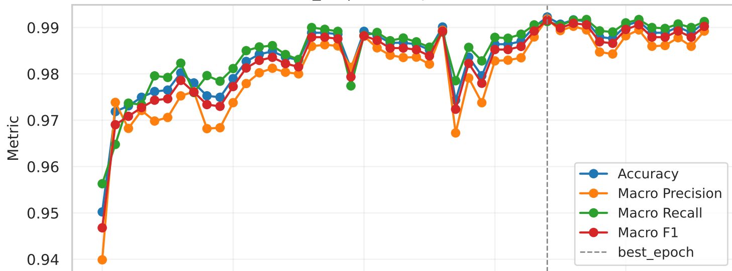
efficientnet_b1 | Accuracy/Precision/Recall/F1
