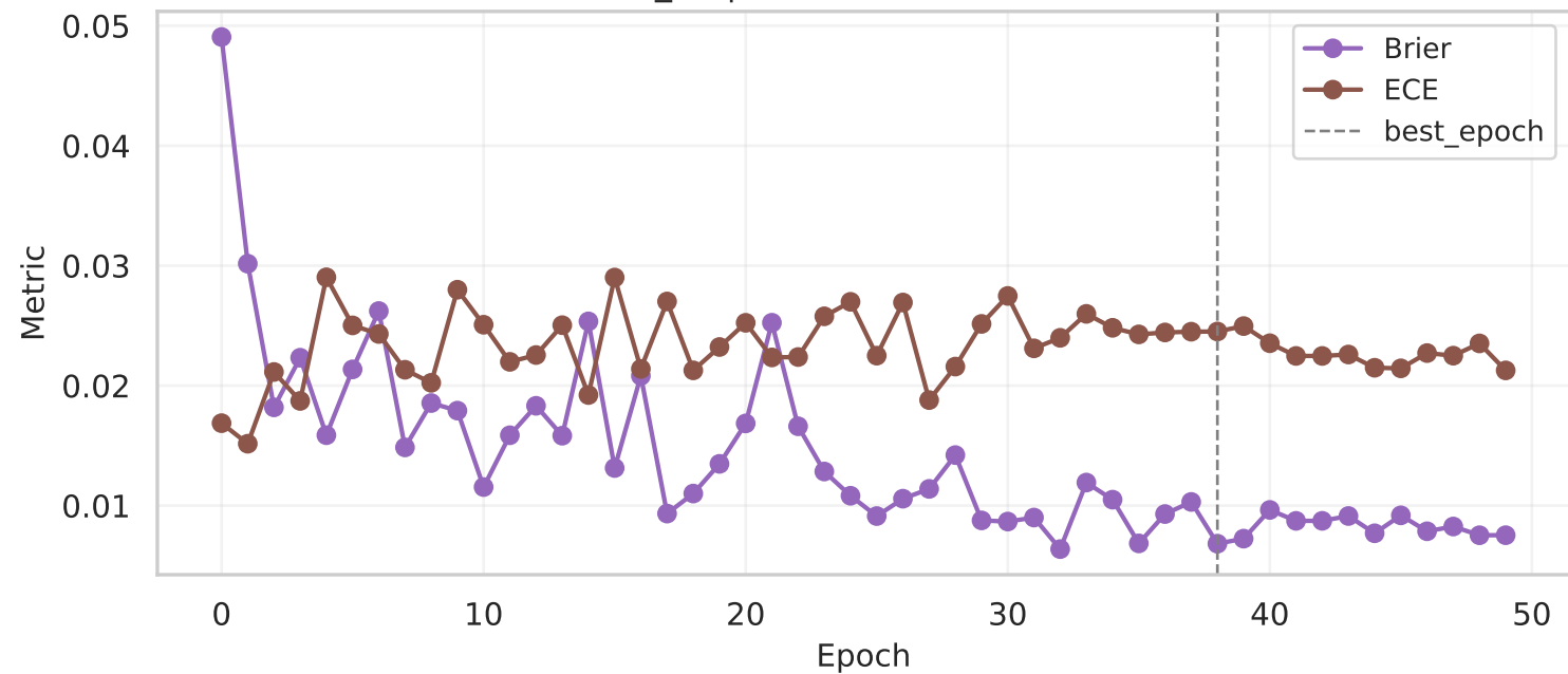
efficientnet_b2 | Calibration metrics (Brier/ECE)
