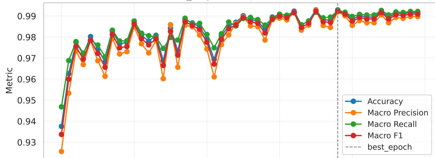
efficientnet_b2 | Accuracy/Precision/Recall/F1
