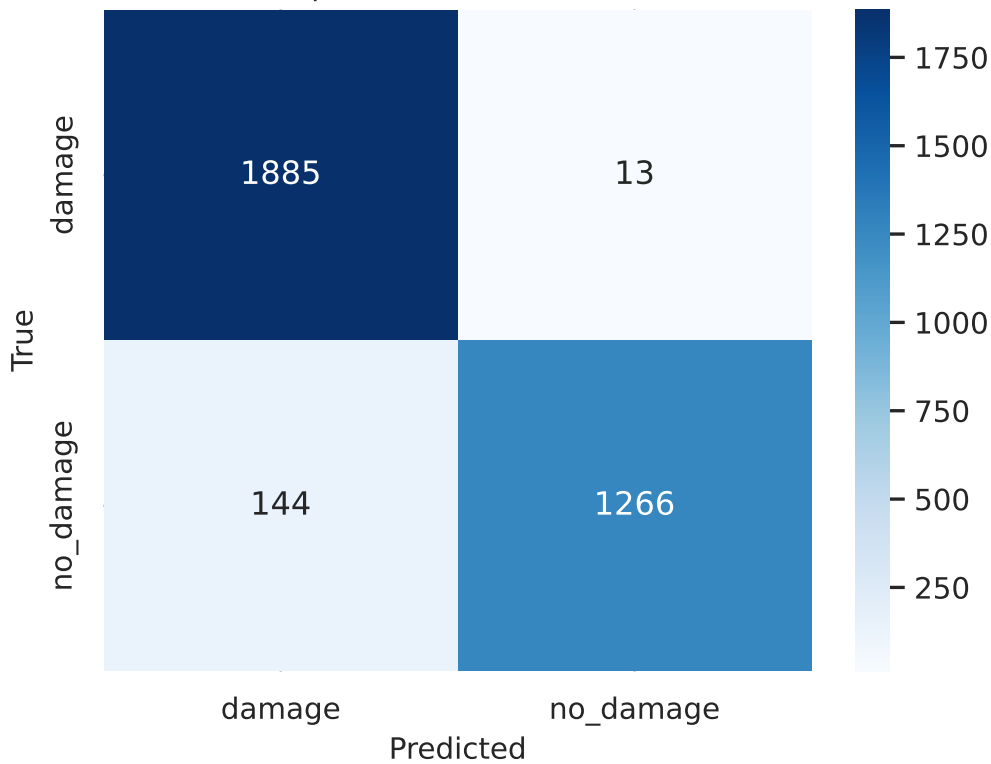
resnet34 | test Confusion (calibrated)
