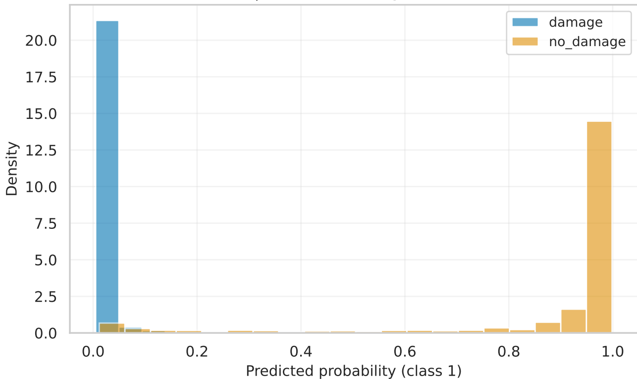
resnet34 | test Score Histogram (calibrated)
