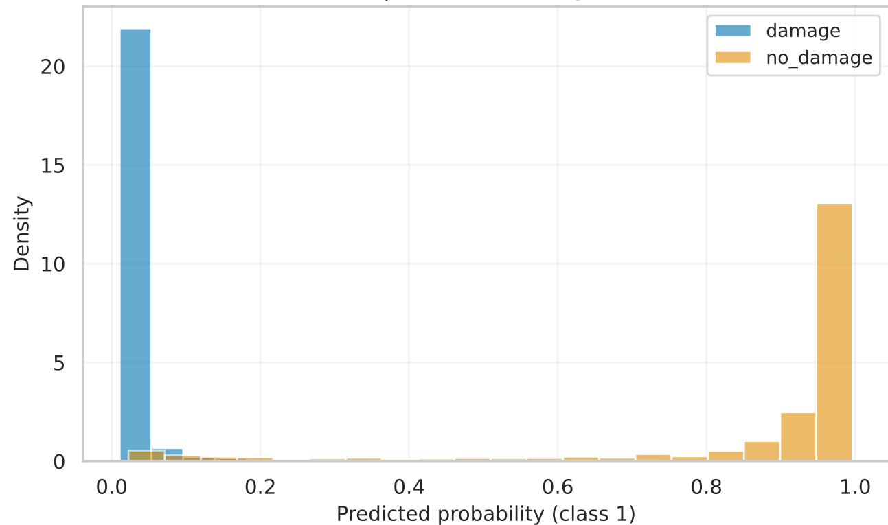
resnet34 | test Score Histogram (raw)
