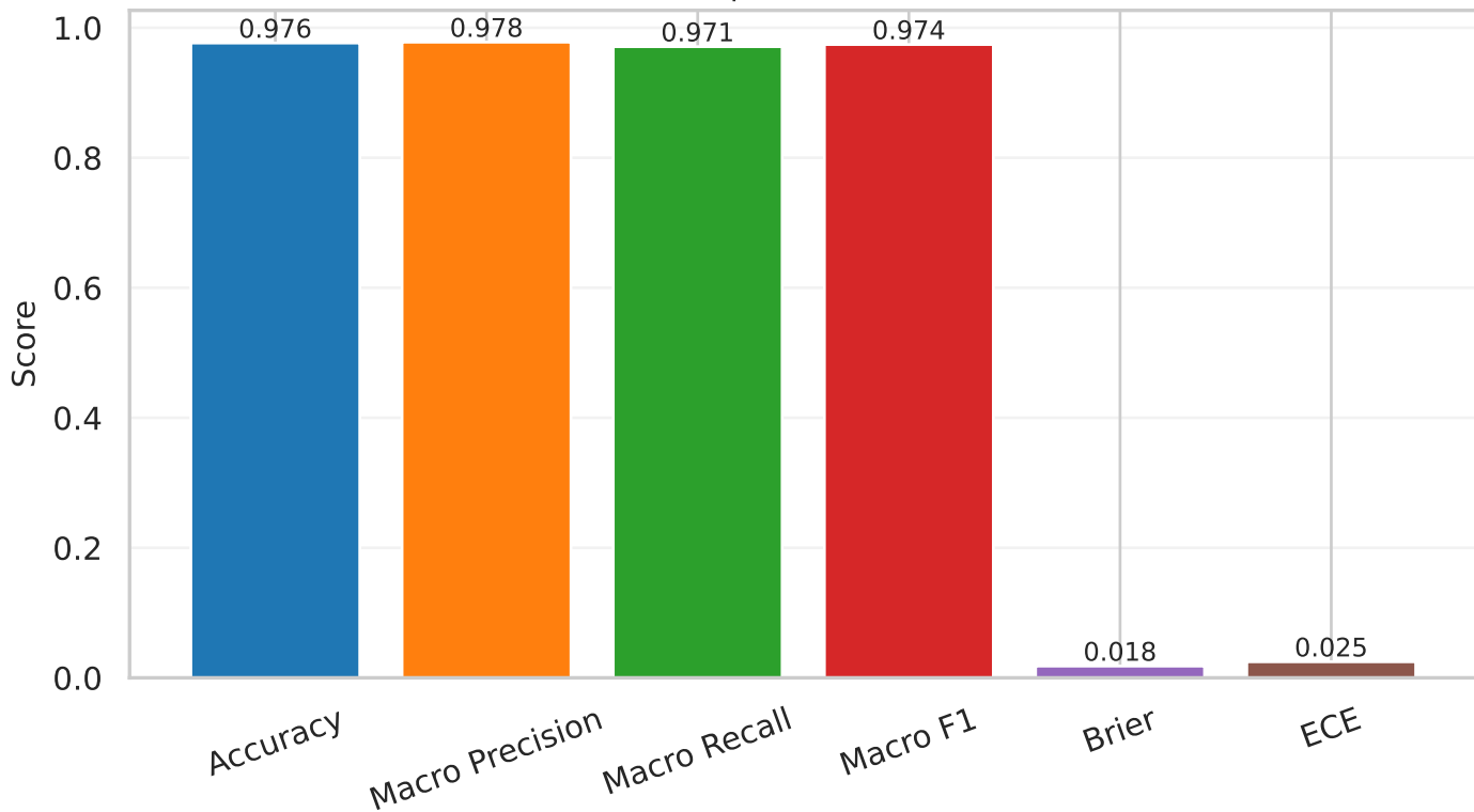
resnet34 | val (raw) metrics
